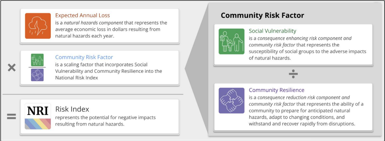
Figure 3: FEMA NRI
