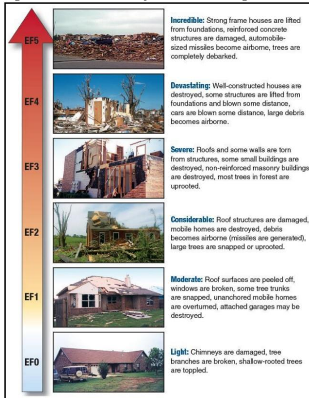
Figure 5: Enhanced Fujita Scale Damage Estimates
